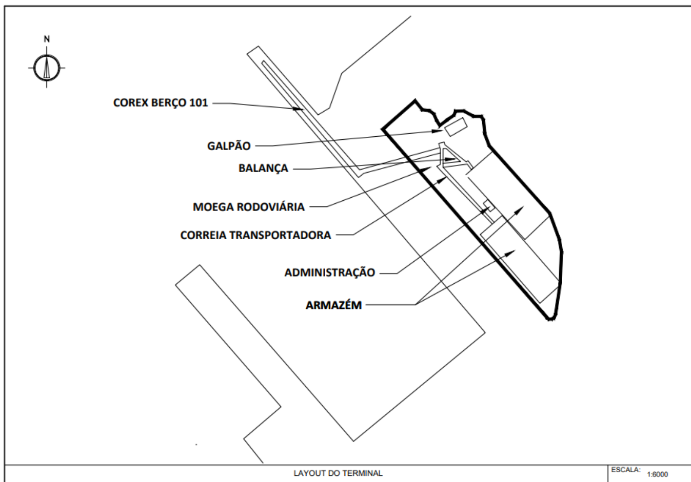
Figura 2 – Layout do Terminal.
